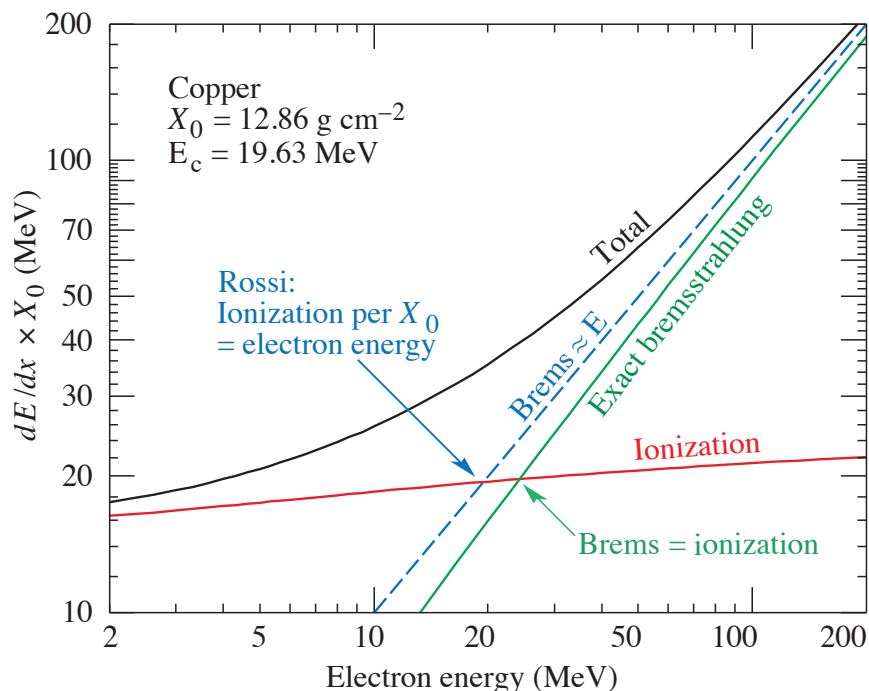
Figure 34.13: Two definitions of the critical energy E_c .
